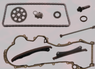
febi 100754 Ref. OE 55261264 S1 Para: Alfa Romeo, Chevrolet, Citroën, FIAT, Ford, Lancia, Opel, Peugeot, Suzuki, Vauxhall
